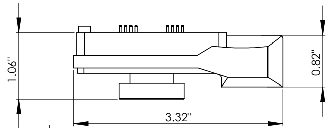
CONNECTOR DETAIL SCALE: 2:1
