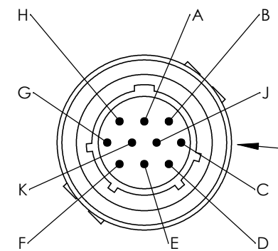
DETAIL END VIEW PIN LOCATION SCALE 2:1 AMPHENOL P/N: PT06E-12-10P
