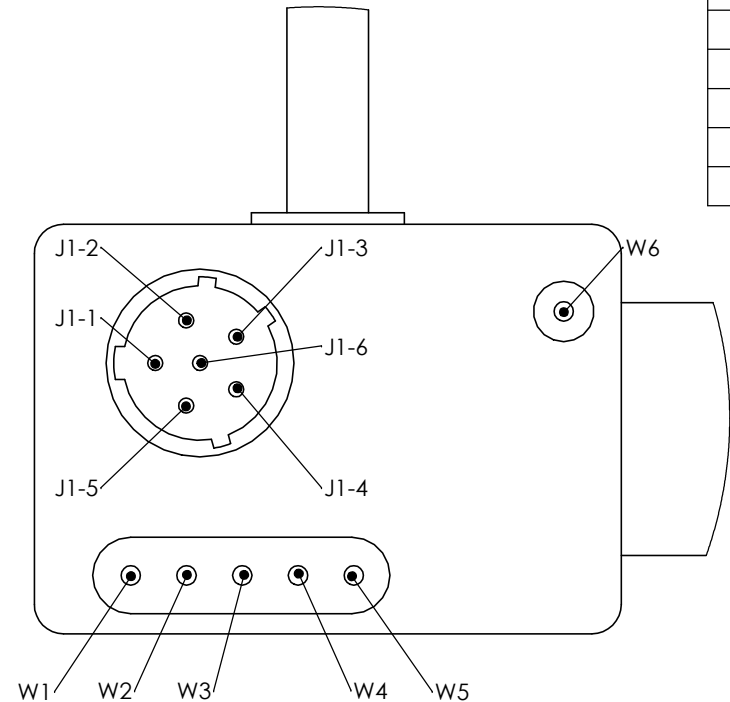
DETAIL VIEW PIN LOCATION SCALE 2:1
